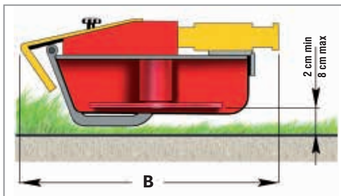
FALK 6/7 Monolama FALK 6/7 Single-blade FALK 6/7 Einzelmesser FALK 6/7 Mono hélice FALK 6/7 Lame-unique
